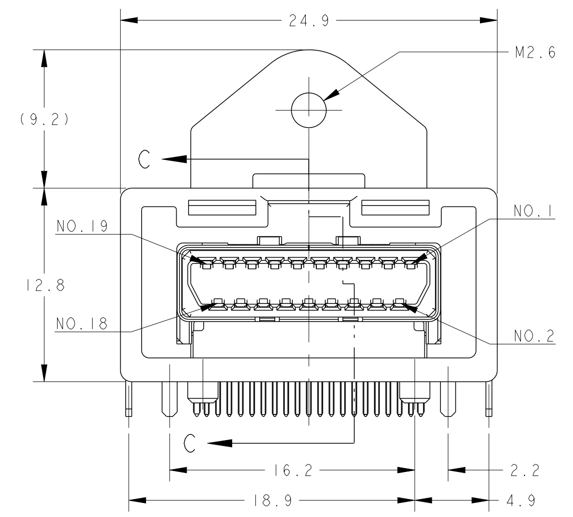
2138755-1 (WITH FLANGE)
