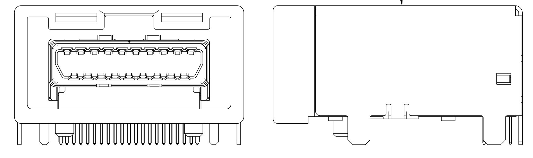
2138755-2 (WITHOUT FLANGE)
