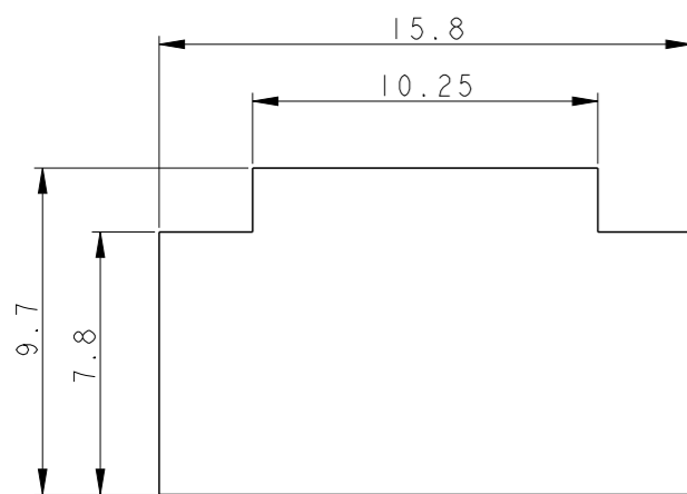
RECOMMENDED PANEL OPENING DIMENSION
