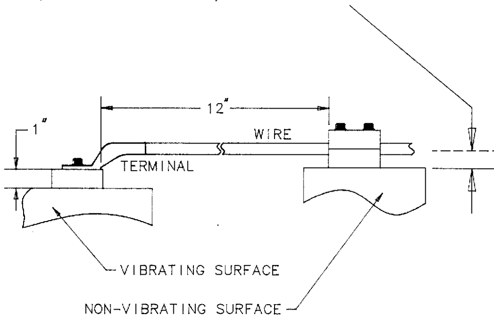
Figure 5 Vibration Mounting Fixtures
