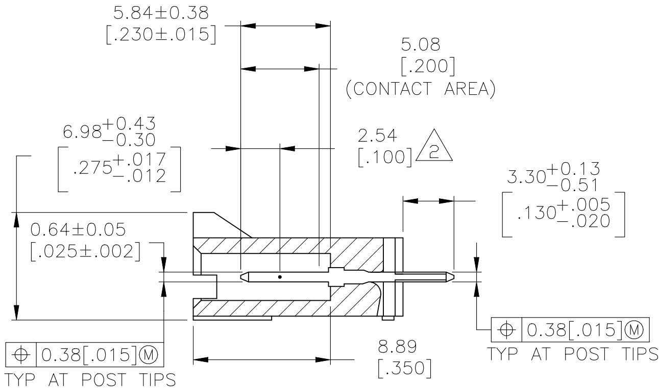
SECTION X-X
